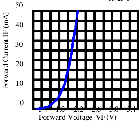
Forward Current & Forward Voltage Ta=25°C
